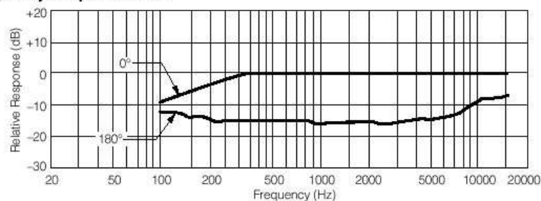
■ Typical Frequency Response Curve
